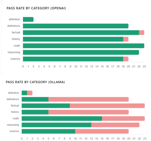
Fig. 7: Per-category pass rates from HTML report — OpenAI vs Ollama
